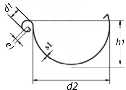
Gutter-cross-section
