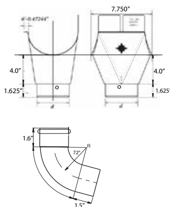
Snap Elbow onto outlet
